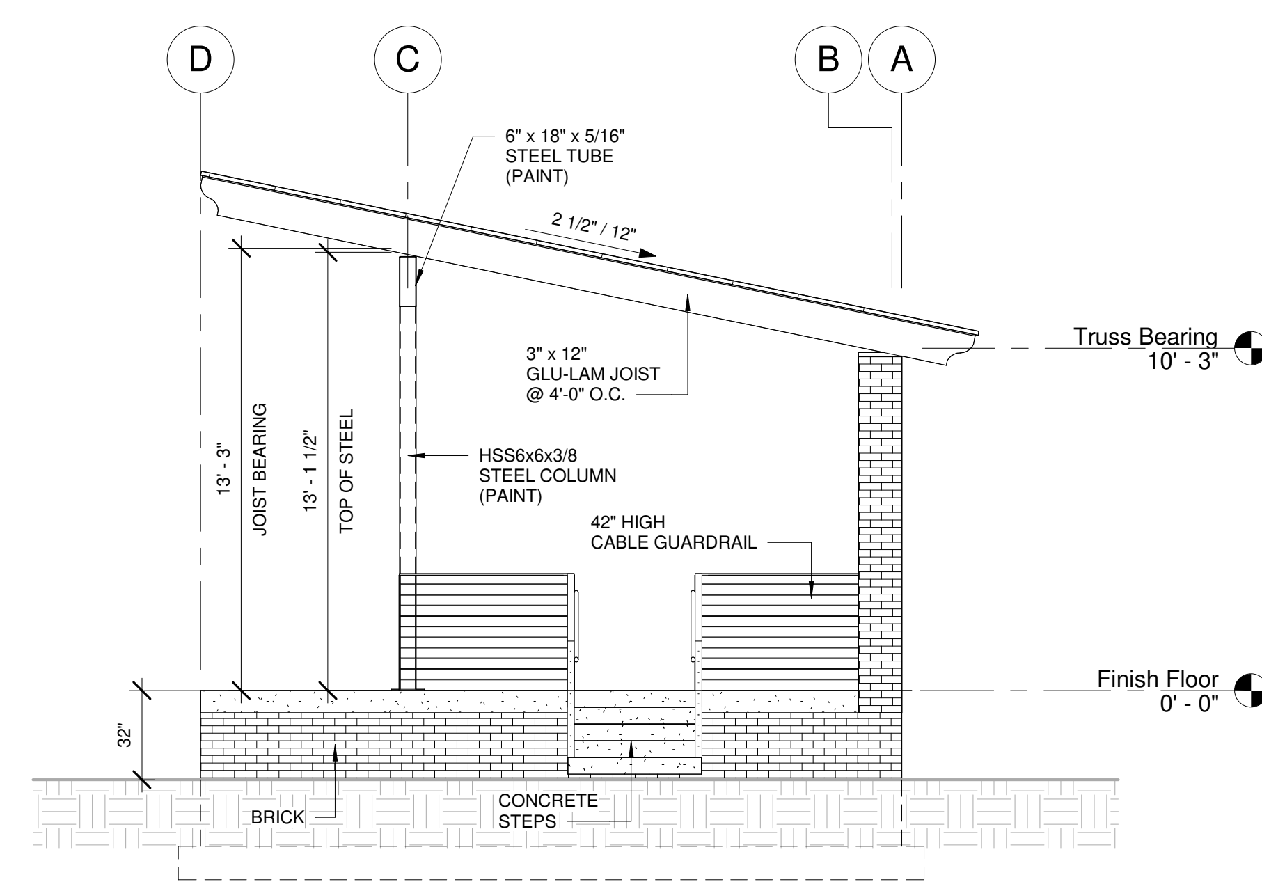
3 East 1/4" = 1'-0"
