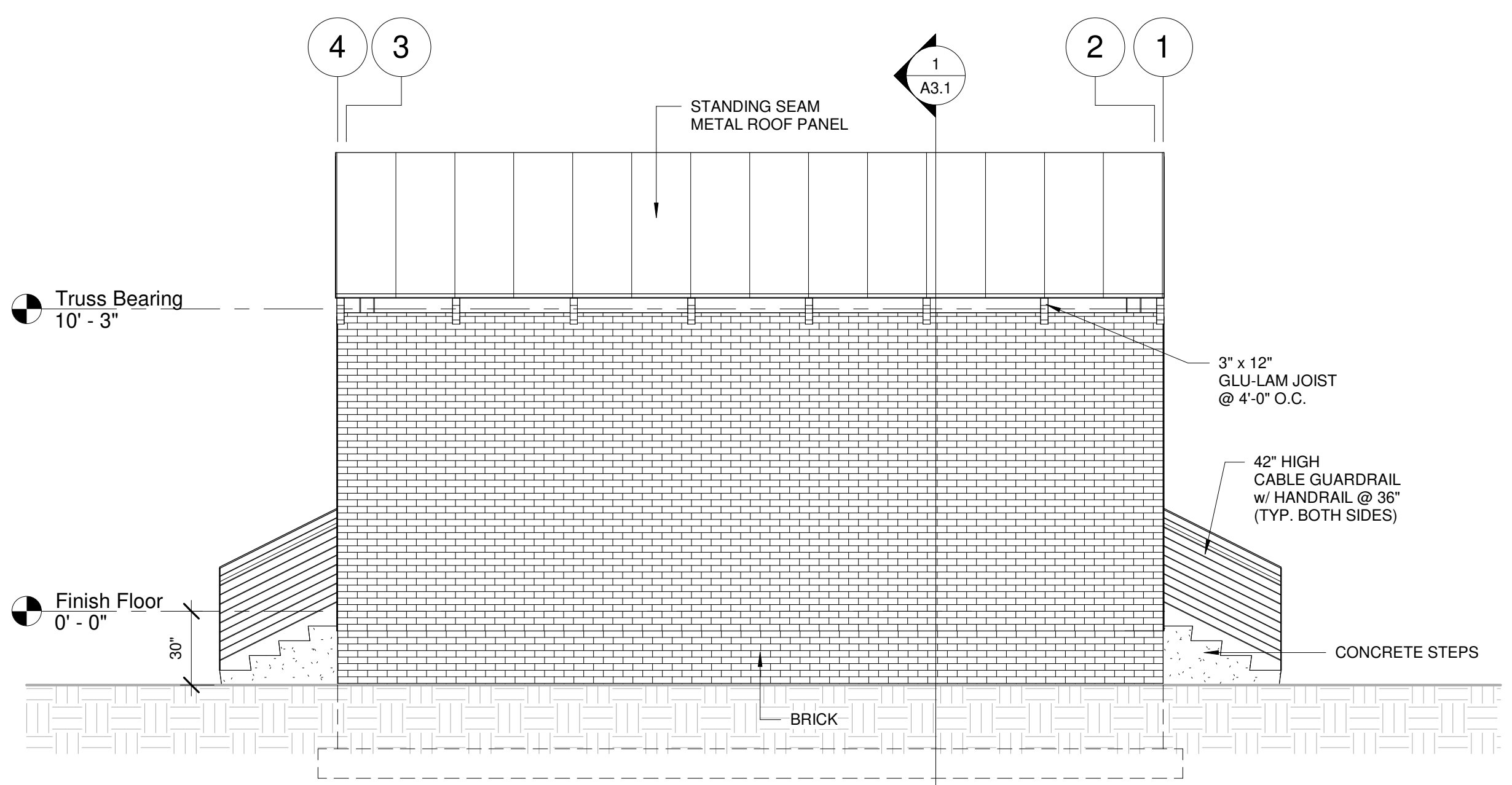
4 North 1/4" = 1'-0"
