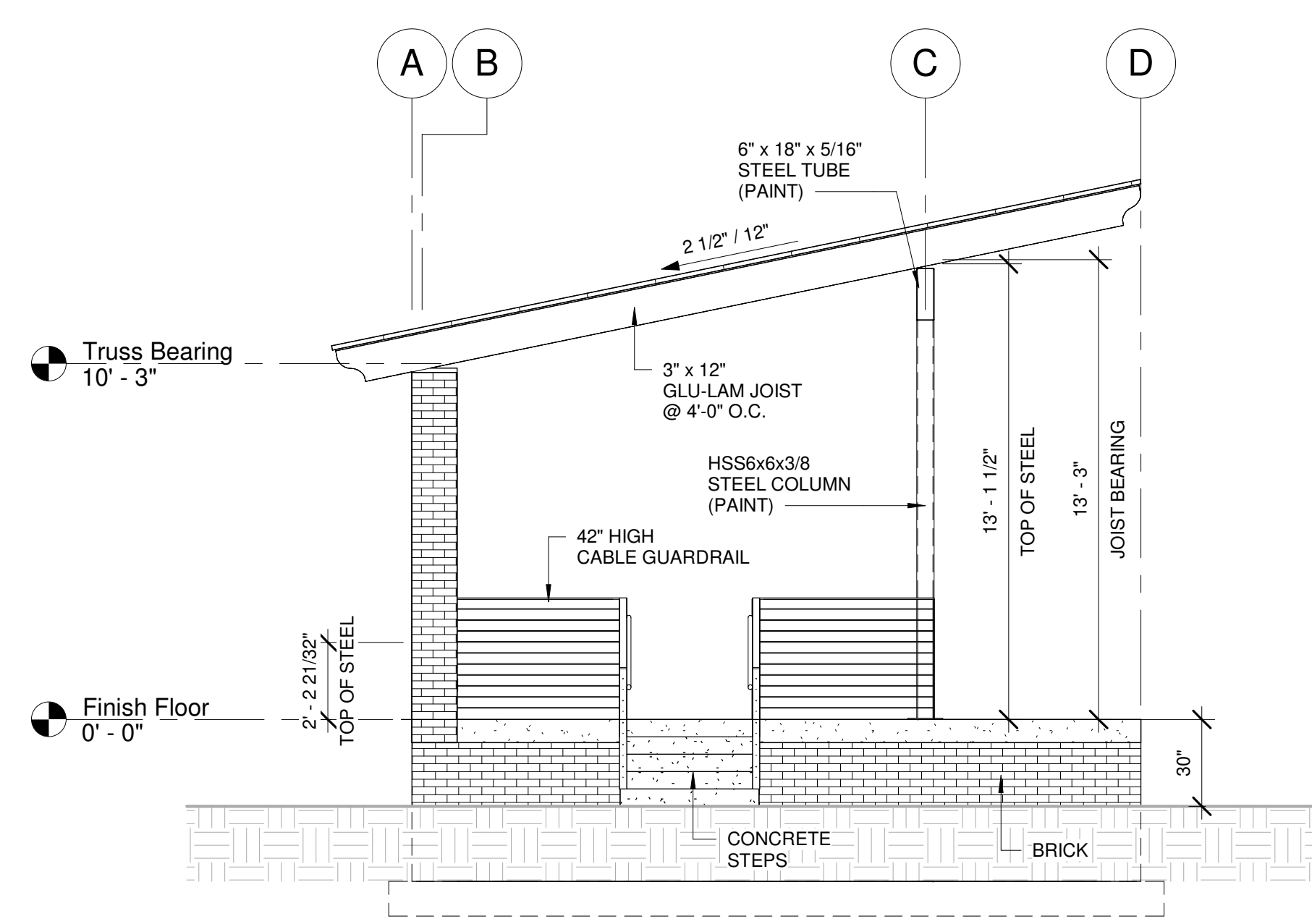
5 West 1/4" = 1'-0"
