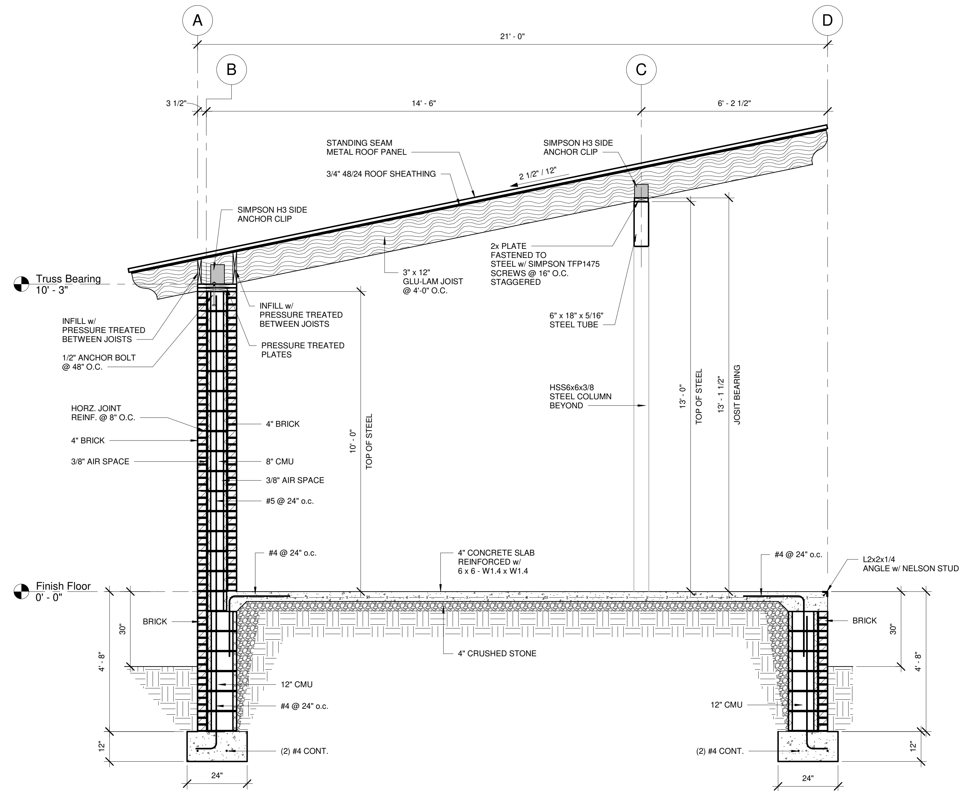
1 BUILDING CROSS SECTION 1/2" = 1'-0"
