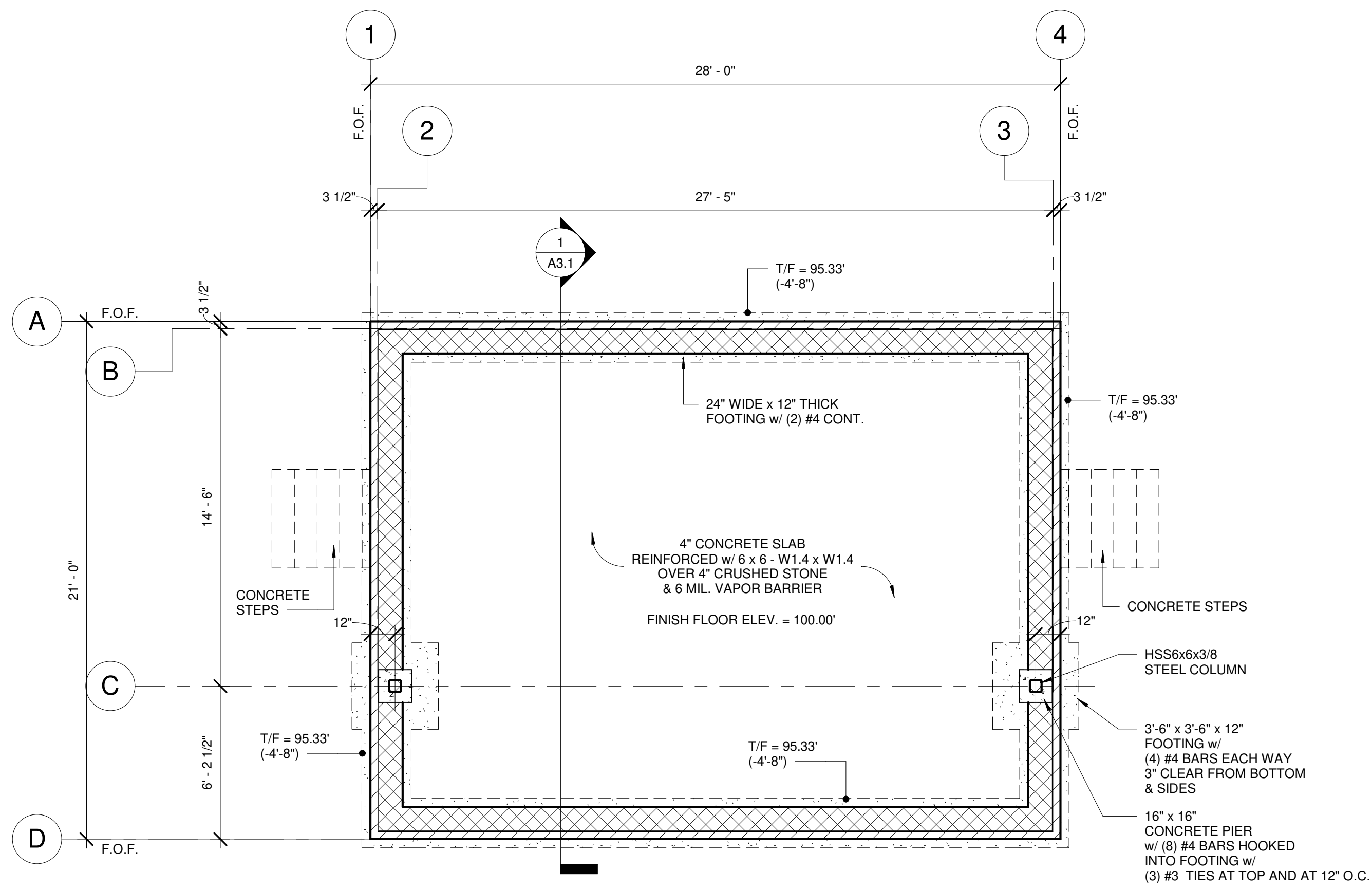
2 FOUNDATION PLAN 1/4" = 1'-0"
