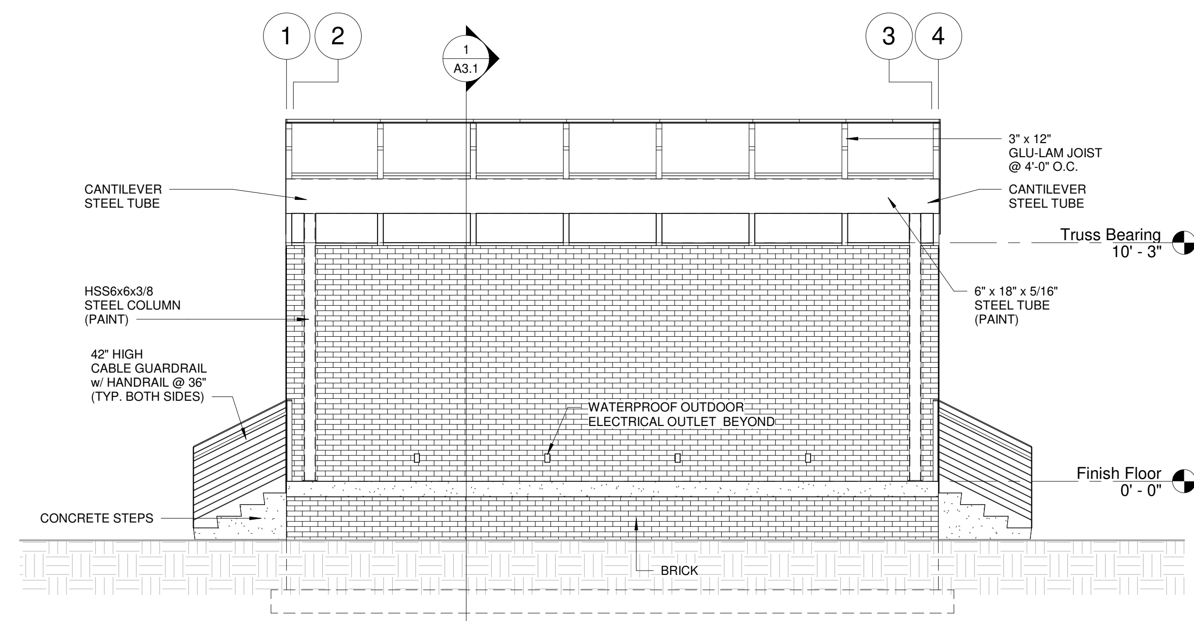
2 South 1/4" = 1'-0"
