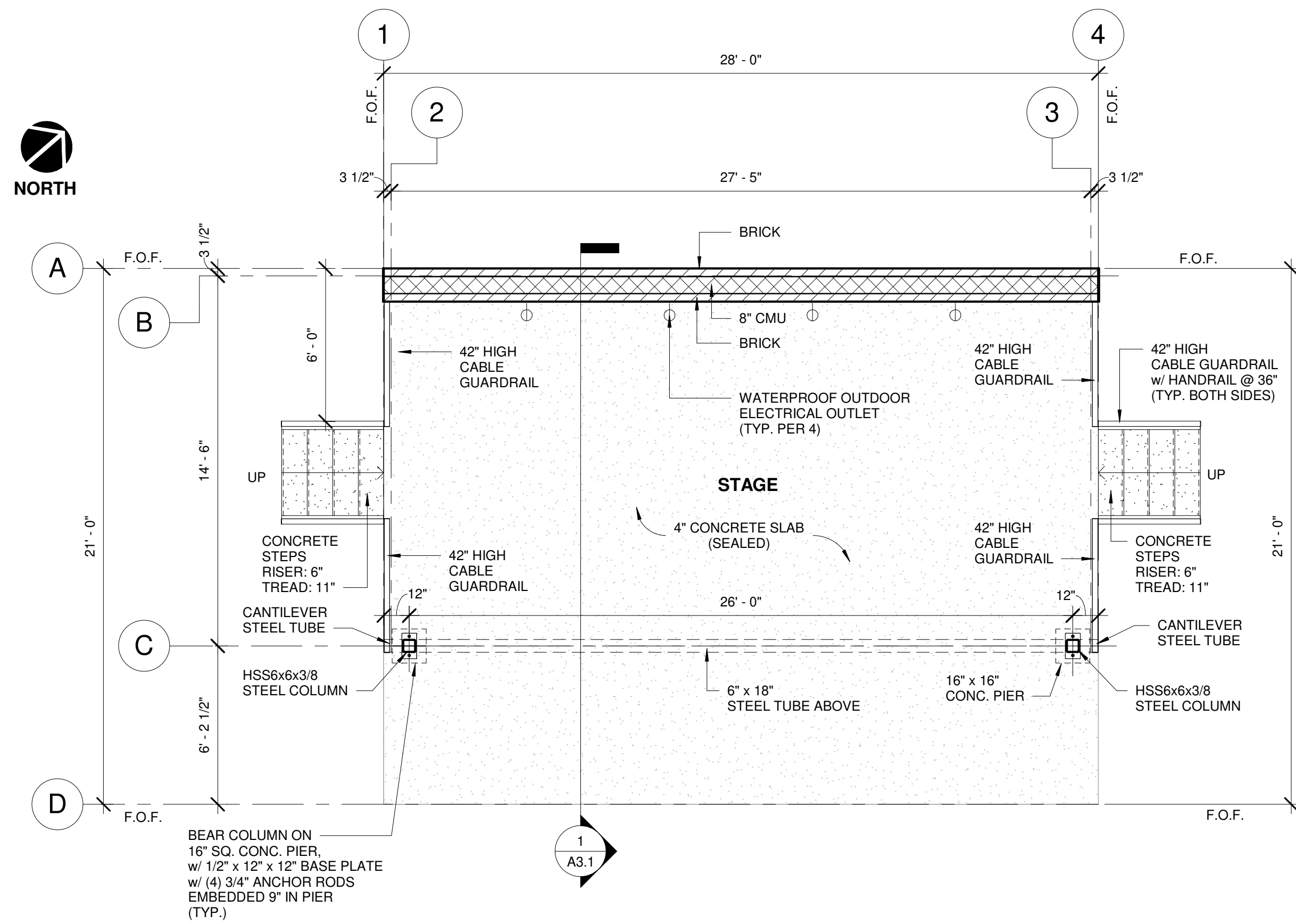
1 FLOOR PLAN 1/4" = 1'-0"
